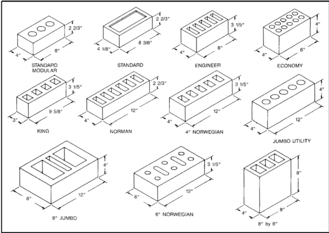
Brick Sizes (Nominal Dimensions)
